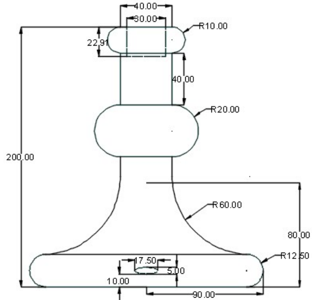
VISTA FRONTAL
